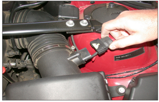
2. Disconnect the mass air sensor electrical connection as shown.
