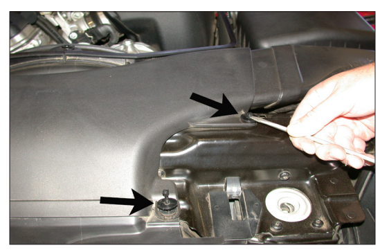
6. Remove the two plastic rivets that secure the air intake scoop as shown.
