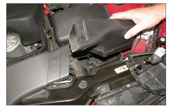
7. Remove the air cleaner air inlet duct as shown.
