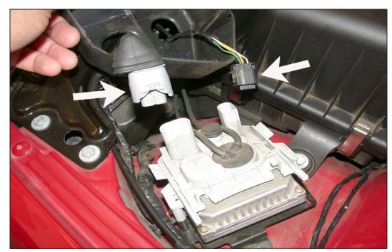
4. Unclip the two electrical connections from the high intensity discharge unit as shown.
