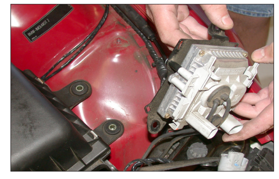
9. Lift up the high intensity discharge unit to gain access to the air cleaner.
