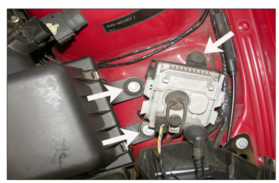
5. Loosen and remove the two bolts and one nut on the high intensity discharge unit as shown. Note: The stock hardware will be reused in a later step.
