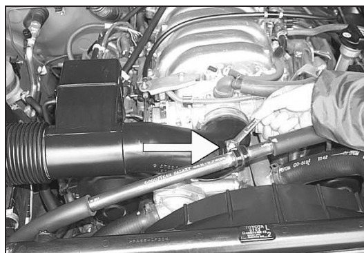
4. Loosen and remove the bolt that secures the AC line to the stock intake tube.
