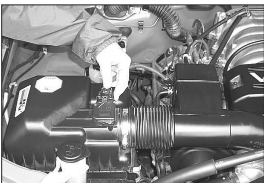
2. Disconnect the mass-air connection.
