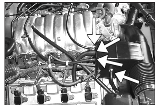
7. Disconnect the four rubber hoses from the engine as shown by the arrows.
