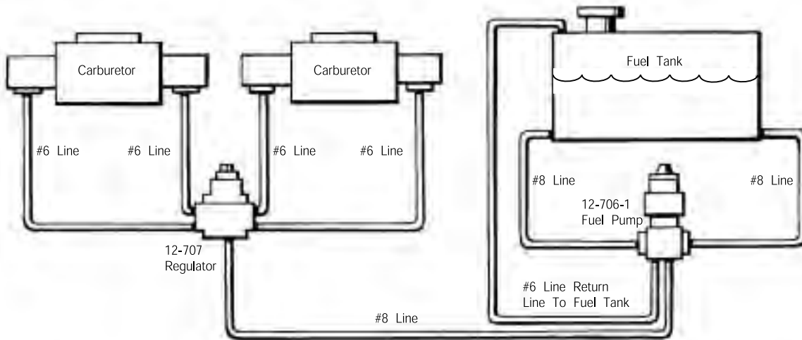
Figure 4 – One (1) #12-706-1 VOLUMAX pump feeding dual carburetors.
